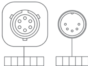
BH300 & BH500 axis and probe for Mitutoyo BH300 and BH500 CMMs
